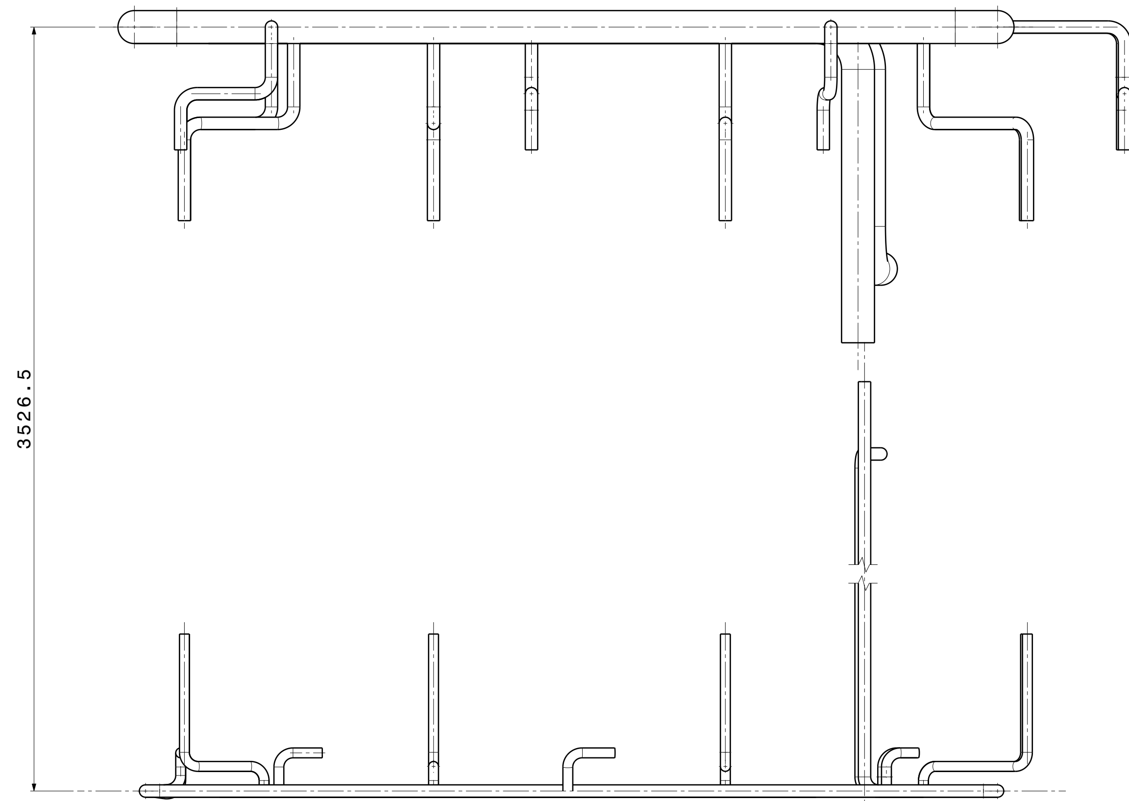
FRONT VIEW
