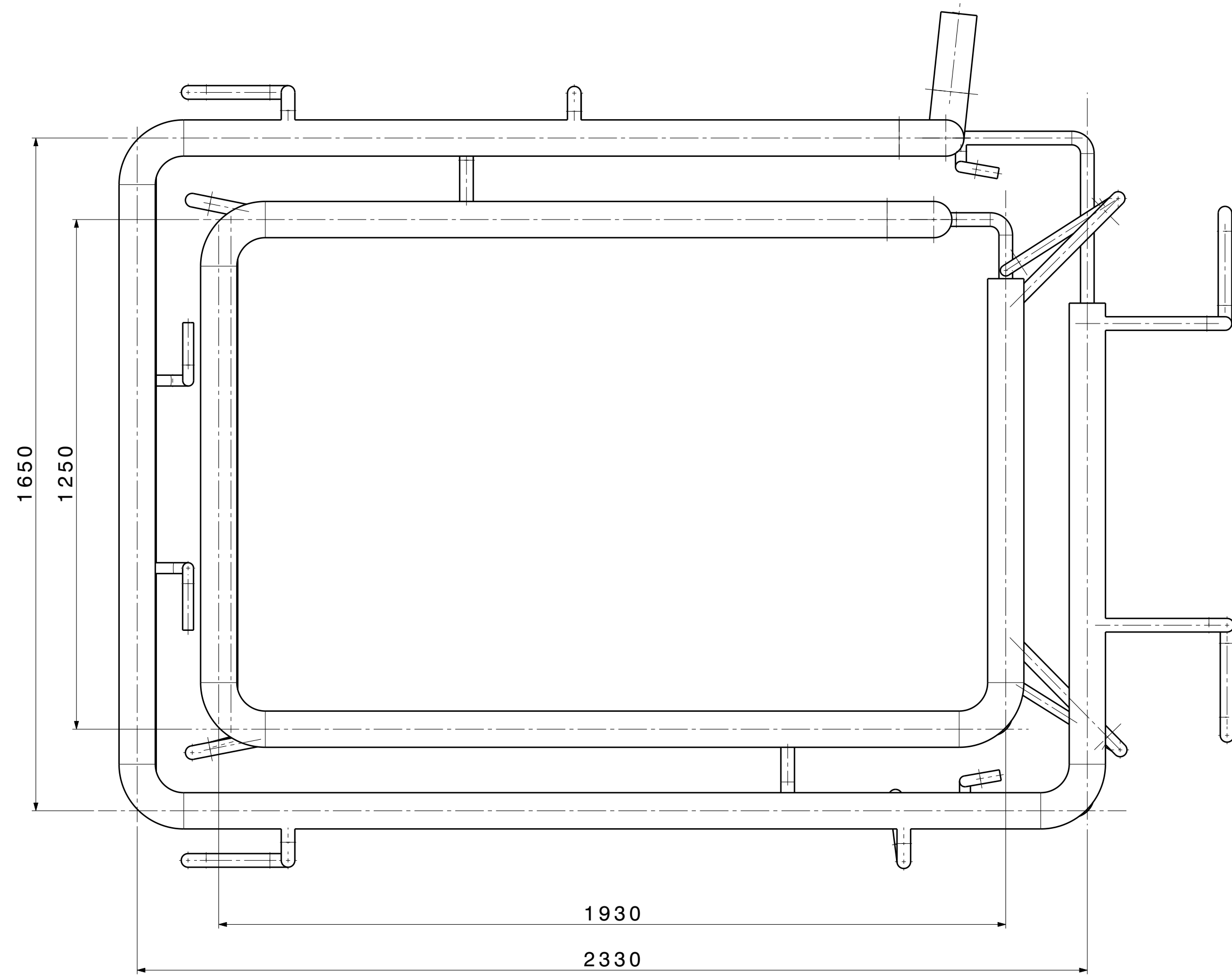
TOP VIEW
