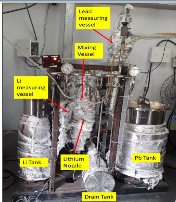
Pb-Li production system at IPR
