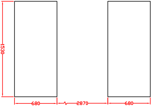
Chiller Foundation Height: 180 mm from Floor Level
