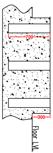
Pump foundation for CTP-2 Pump
