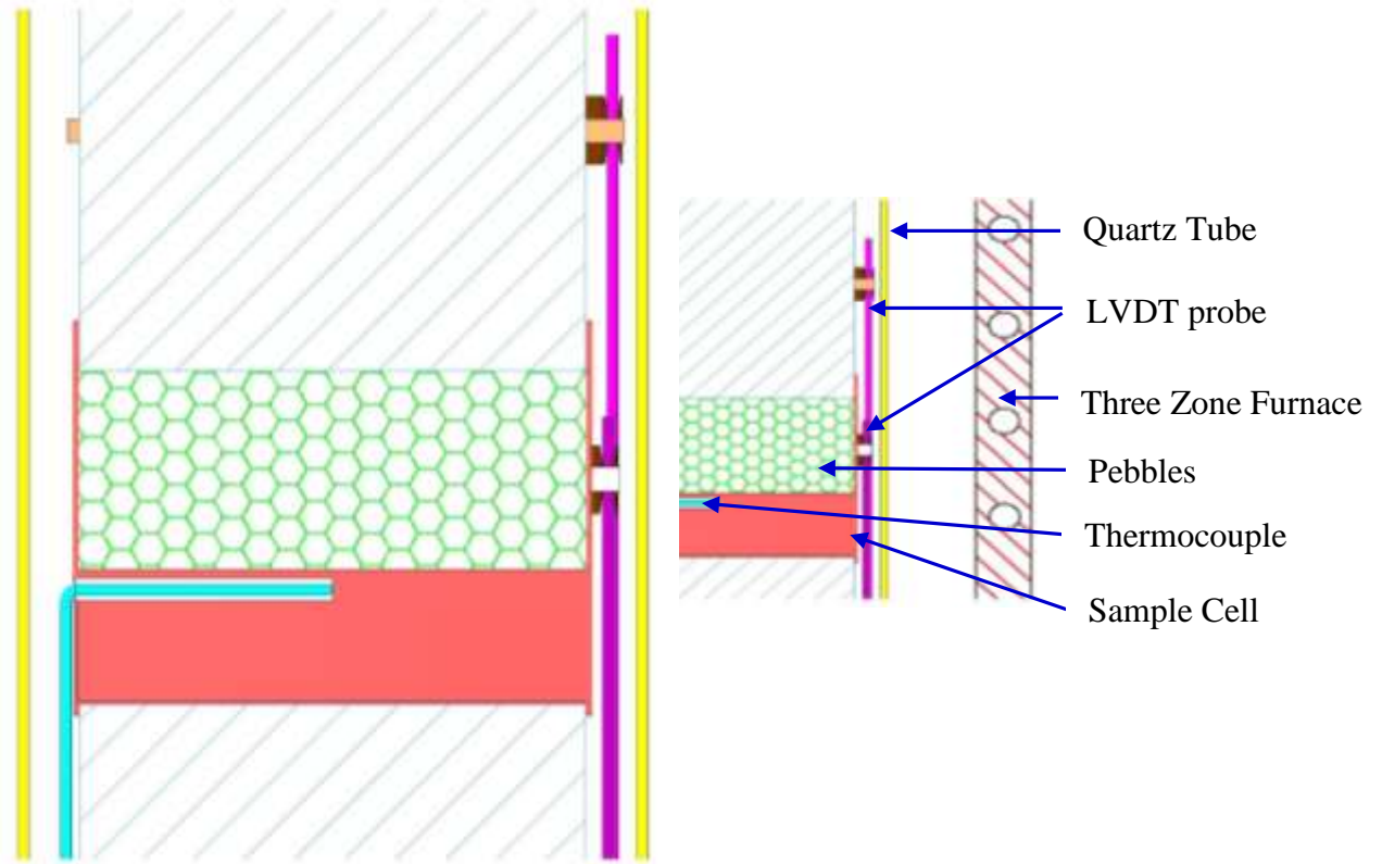
Fig. 2. Schematic of Alternate locations of LVDT
